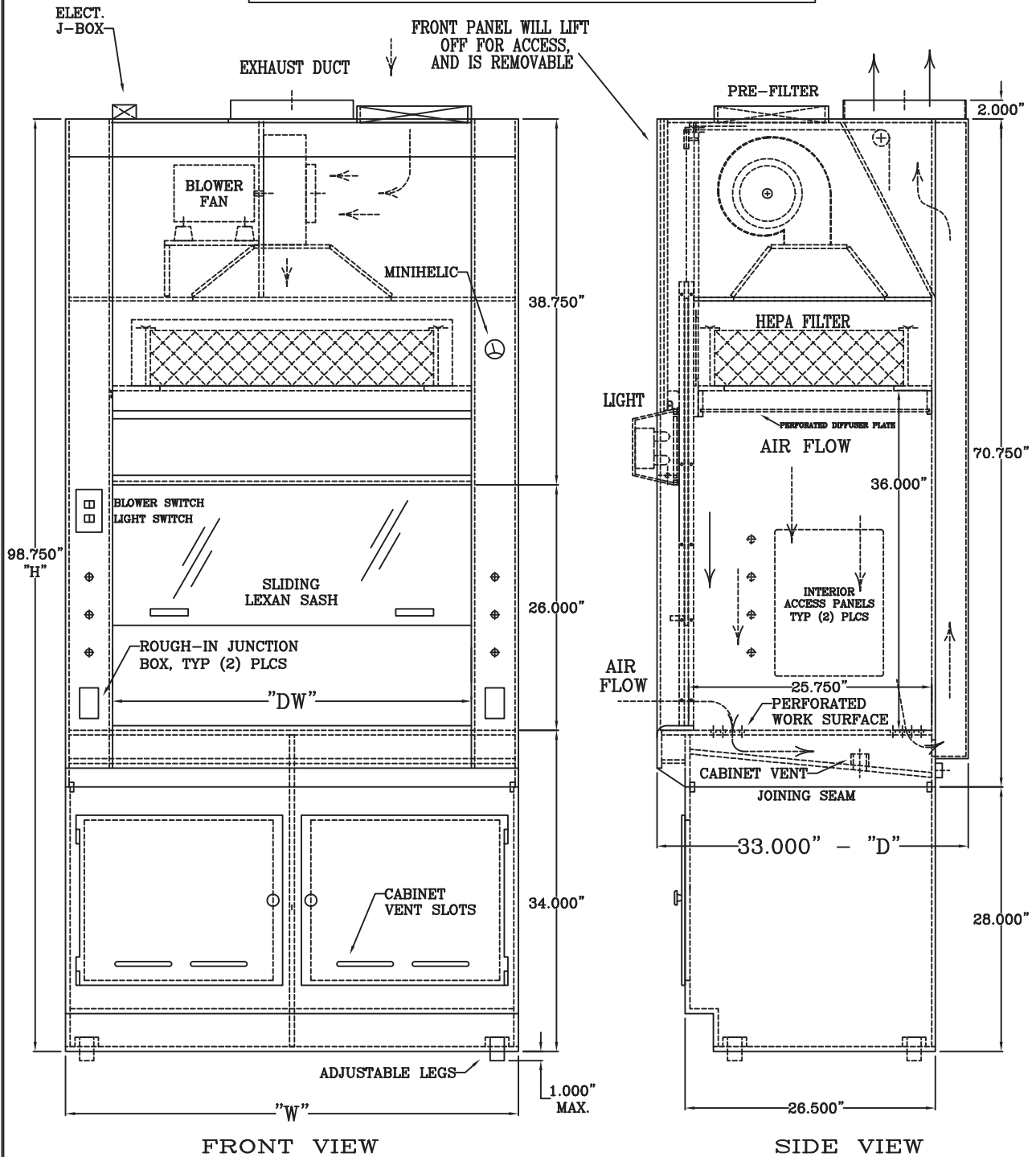
PLASTIC LAMINAR FLOW FUME HOOD
