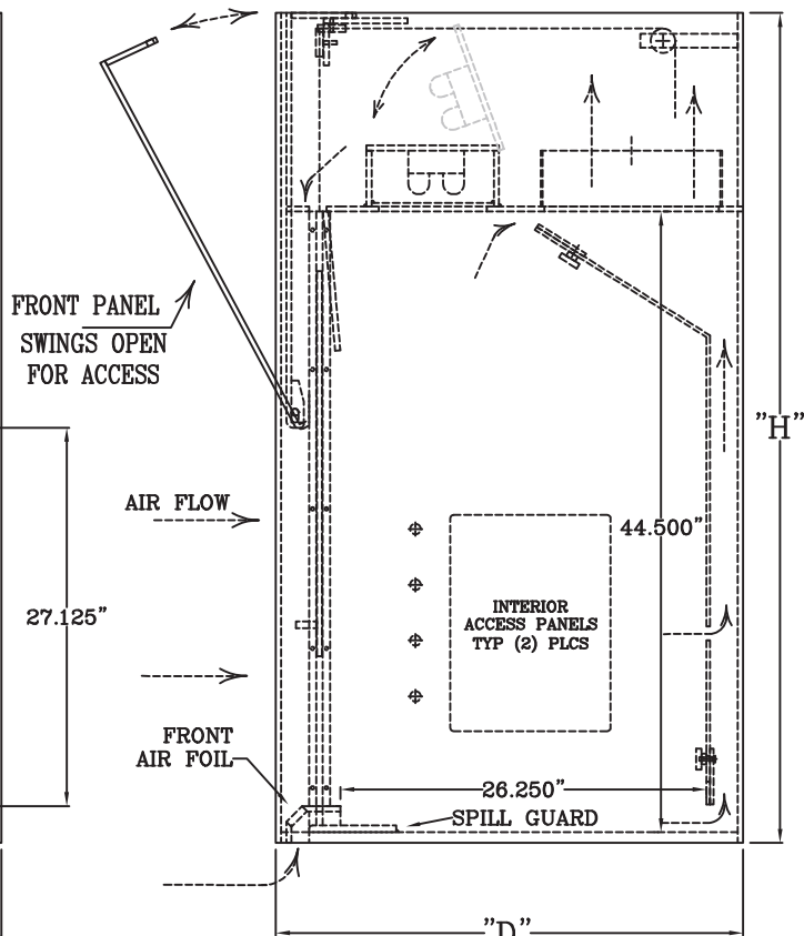
SIDE VIEW
